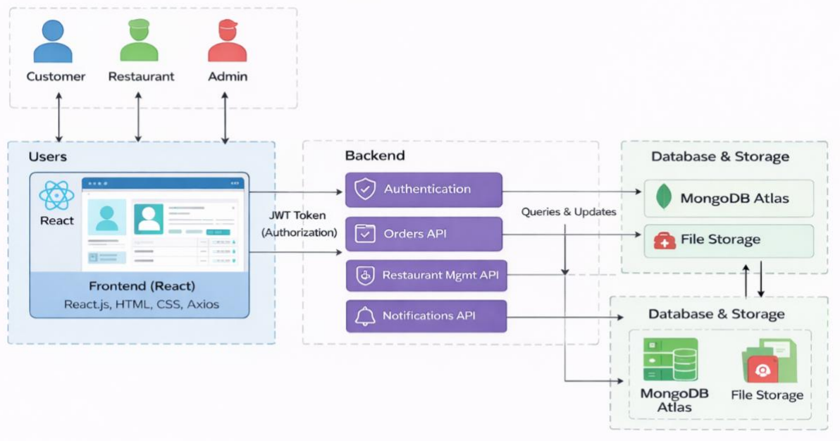
Figure-1: Architecture and data flow of the OrderOnTheGo MERN-stack food ordering platform.
